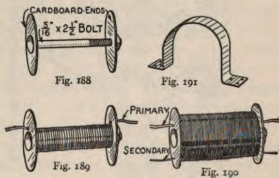
FIGS. 188-191. — Details of Induction-Coil.
